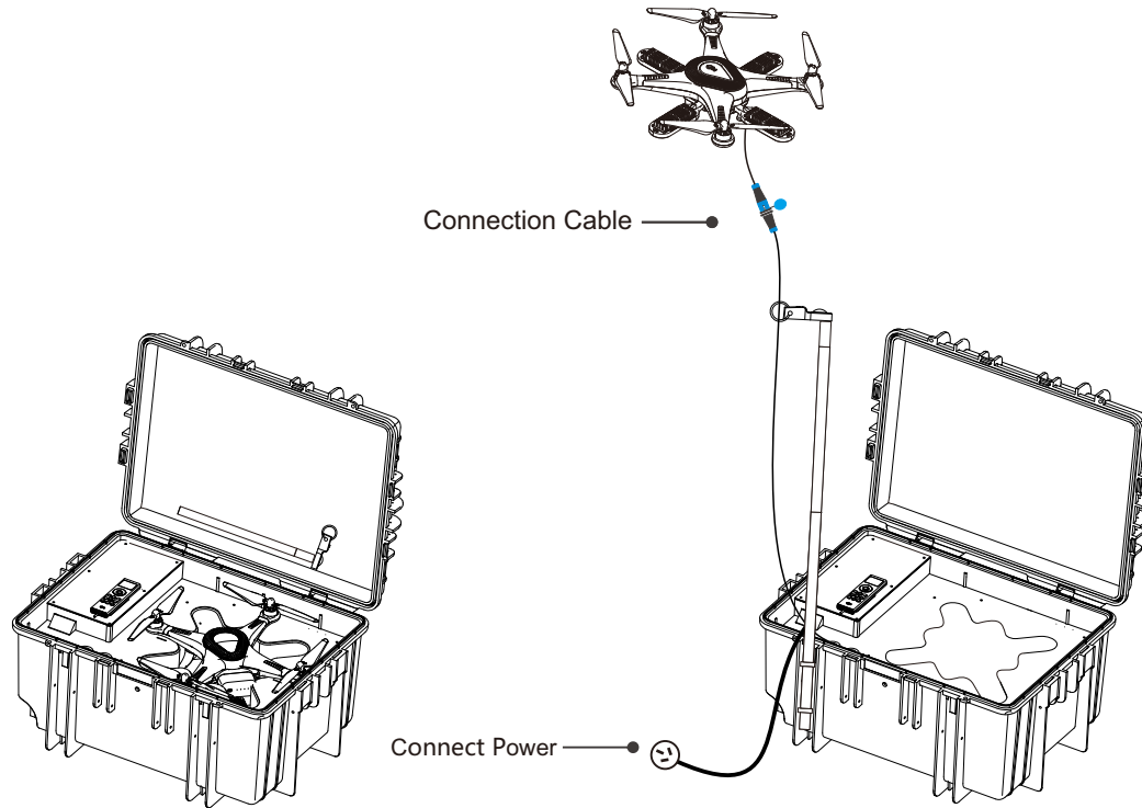
Figure 4-1:Schematic Diagram Of The Initial State Of The System Figure 4-2:Schematic Diagram Of The Final Connection Of The System
