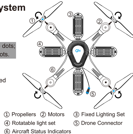
Figure 2:Schematic diagram of the lighting drone components
