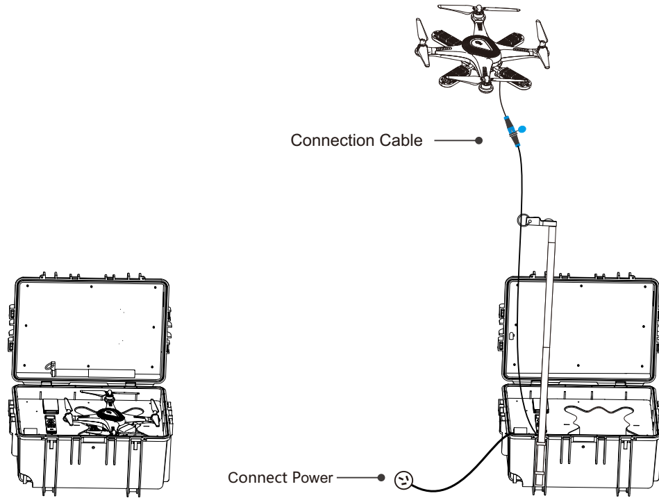
Figure 4-1: Schematic Diagram Of The Initial State Of The System Figure 4-2: Schematic Diagram Of The Final Connection Of The System
