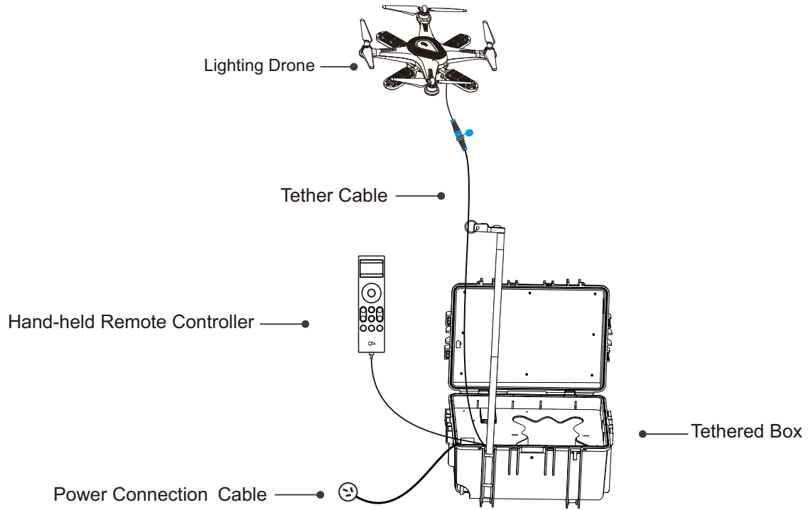
Figure 1:Schematic Diagram Of System Components
