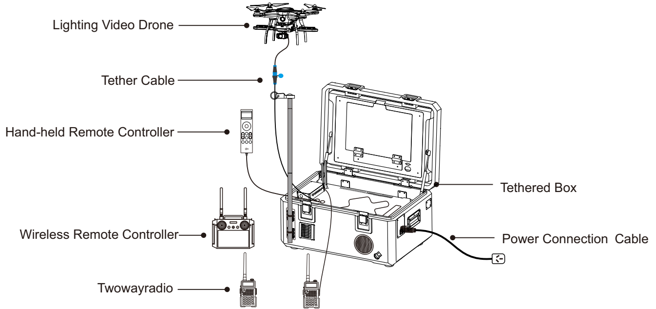
Figure 1:Schematic Diagram Of System Components
