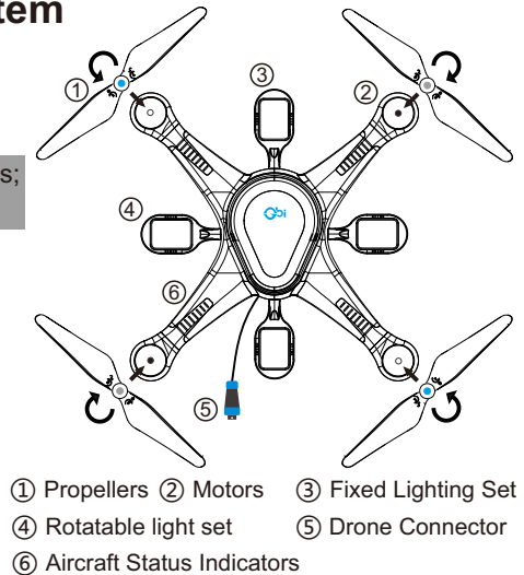
Figure 2:Schematic diagram of the lighting drone components
