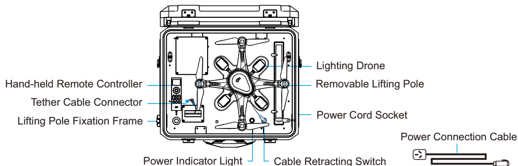
Figure 3: Schematic Diagram Of The Components Of The Tethered Box
