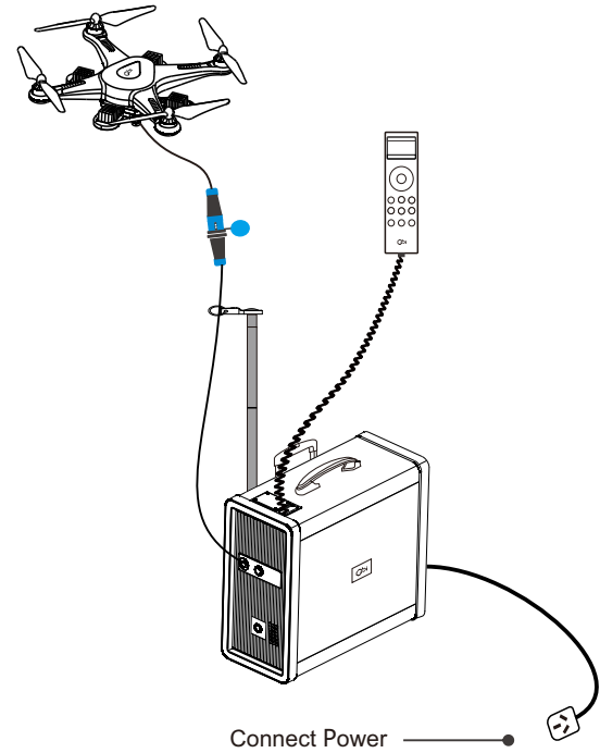
Figure 4-1:Schematic Diagram Of The Initial State Of The System Figure 4-2:Schematic Diagram Of The Final Connection Of The System
