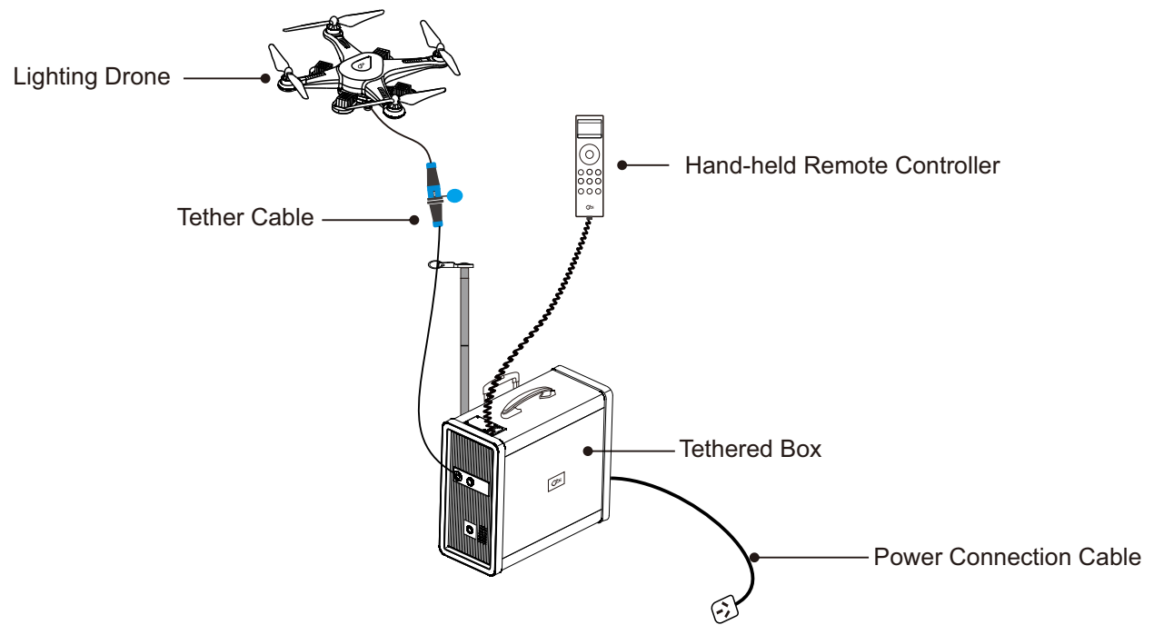
Figure 1: Schematic Diagram Of System Components
